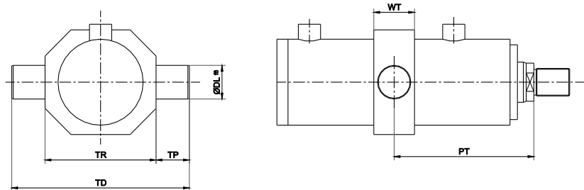
DIMENSIONAL DETAILS
