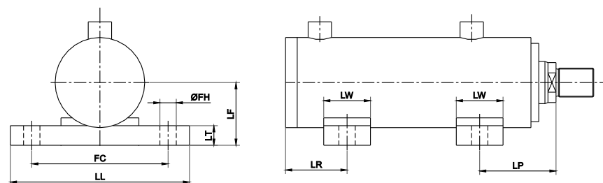
DIMENSIONAL DETAILS
